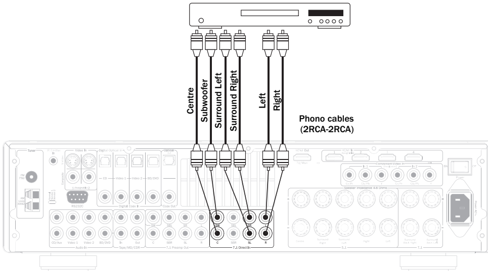
DVD-A player or SACD multi-channel player 5.1 connections
